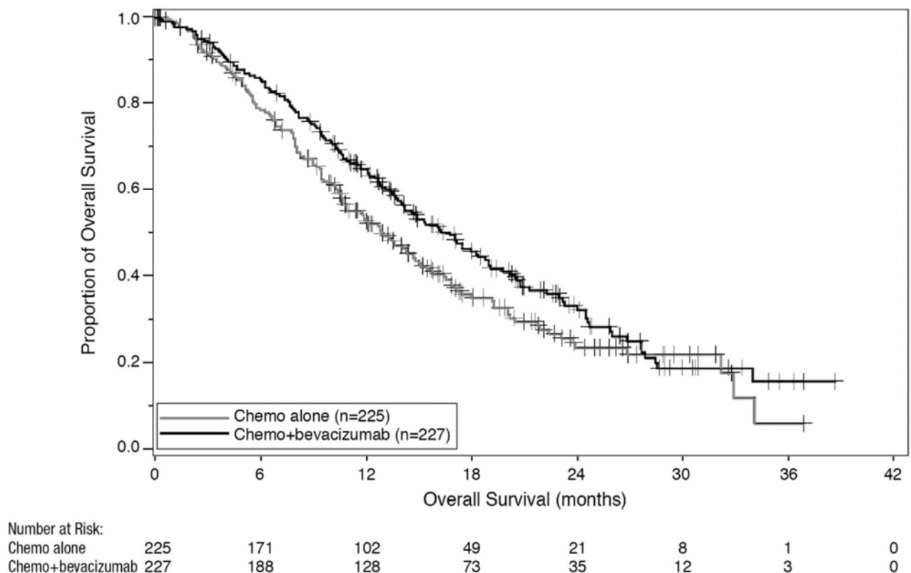
Figure 5: Kaplan-Meier Curves for Overall Survival in Persistent, Recurrent, or Metastatic Cervical Cancer in Study GOG-0240
